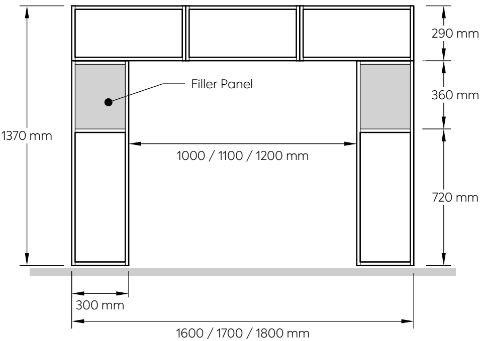
CARCASS FRONT VIEW
