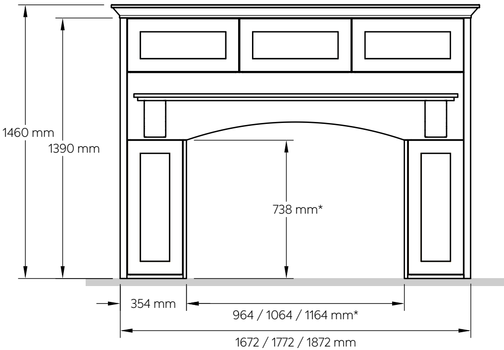
FRONT VIEW
